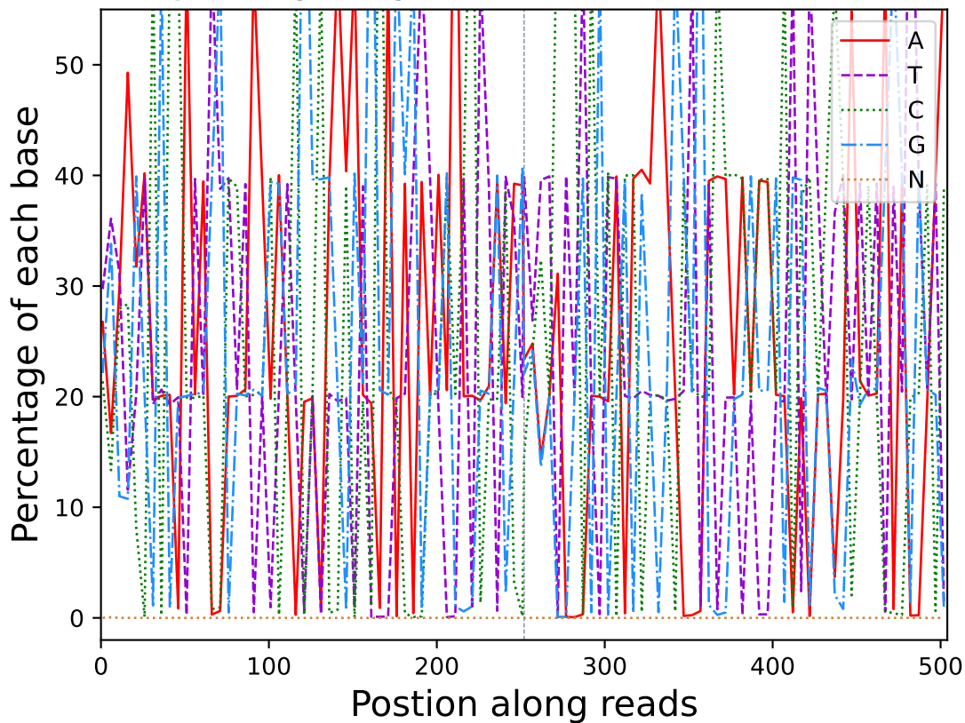
Base percentage along reads (R20122)
